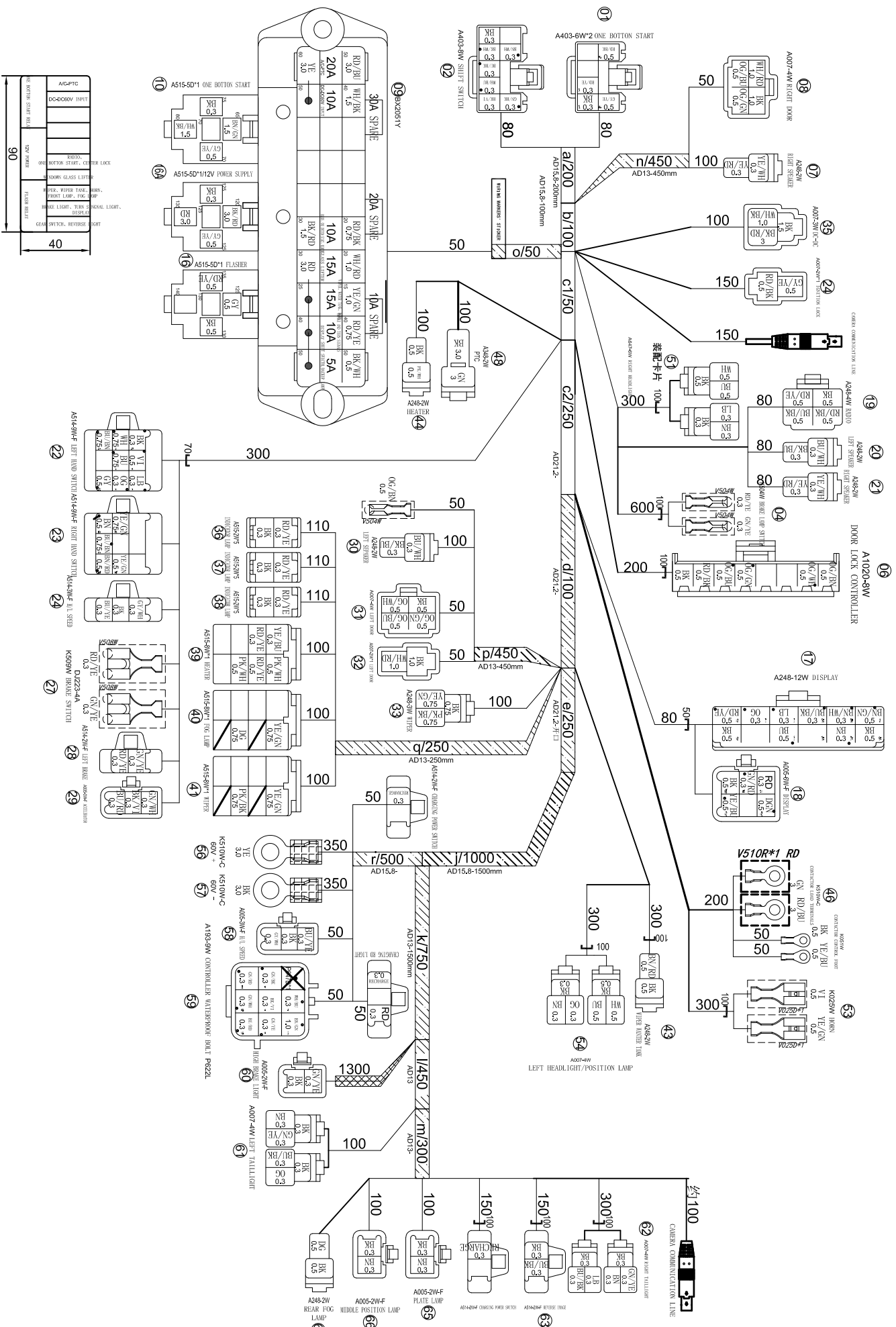
WIRING CONNECTION LINE
